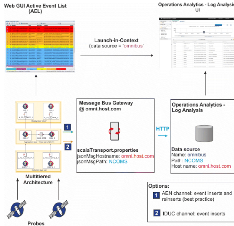
Figure 2. Multitier architecture deployment - Aggregation layer
